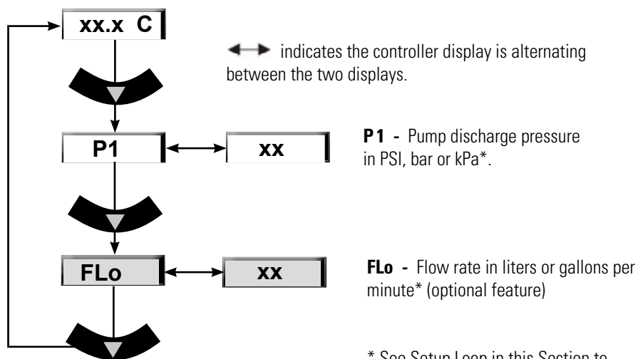
Figure 4-2 Main Loop
