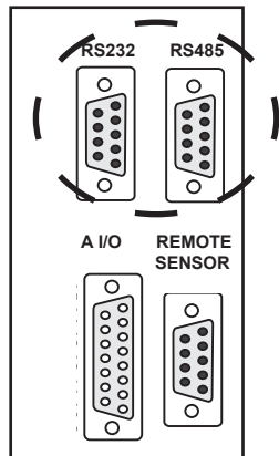
Figure D-1 Connectors
